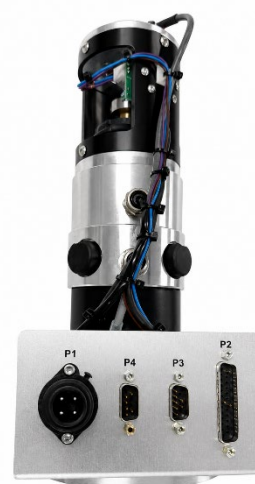
Connector panel — plugs straight into the original arm wiring
